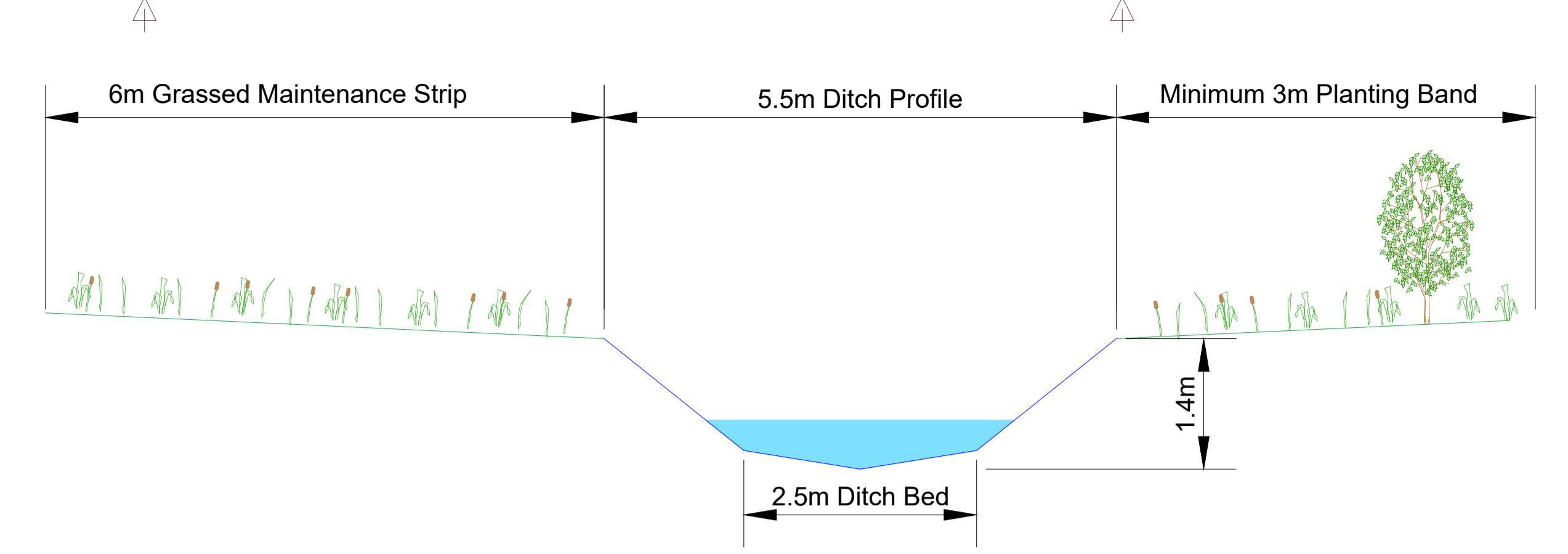
Typical Section (Scale 1:50) All dimensions are approximate
