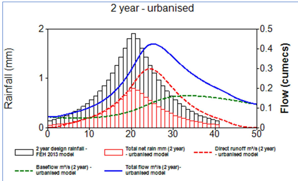
Figure 9 : ReFH2 Generated Hydrograph in Storm Dennis, indicating a 1 in 2 year design hydrograph with a peak flow of 0.43 m 3 /s (read from the blue line and right hand vertical axis).
