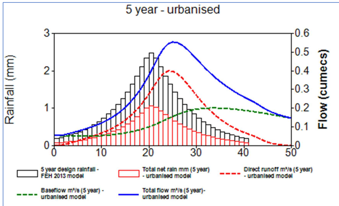
Figure 10: ReFH2 Generated Hydrographs for the 1 in 5 year return period – indicating peak flow rates of 0.56 m 3 /s – read from the blue line the right hand vertical axis.
