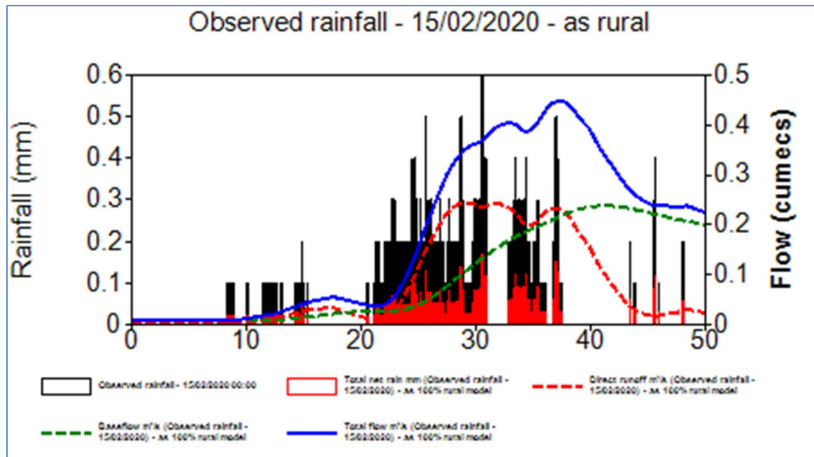
Figure 8: ReFH2 Generated Hydrograph in Storm Dennis, indicating a peak total flow of 0.46 m 3 /s (read from the blue line and right hand vertical axis).
