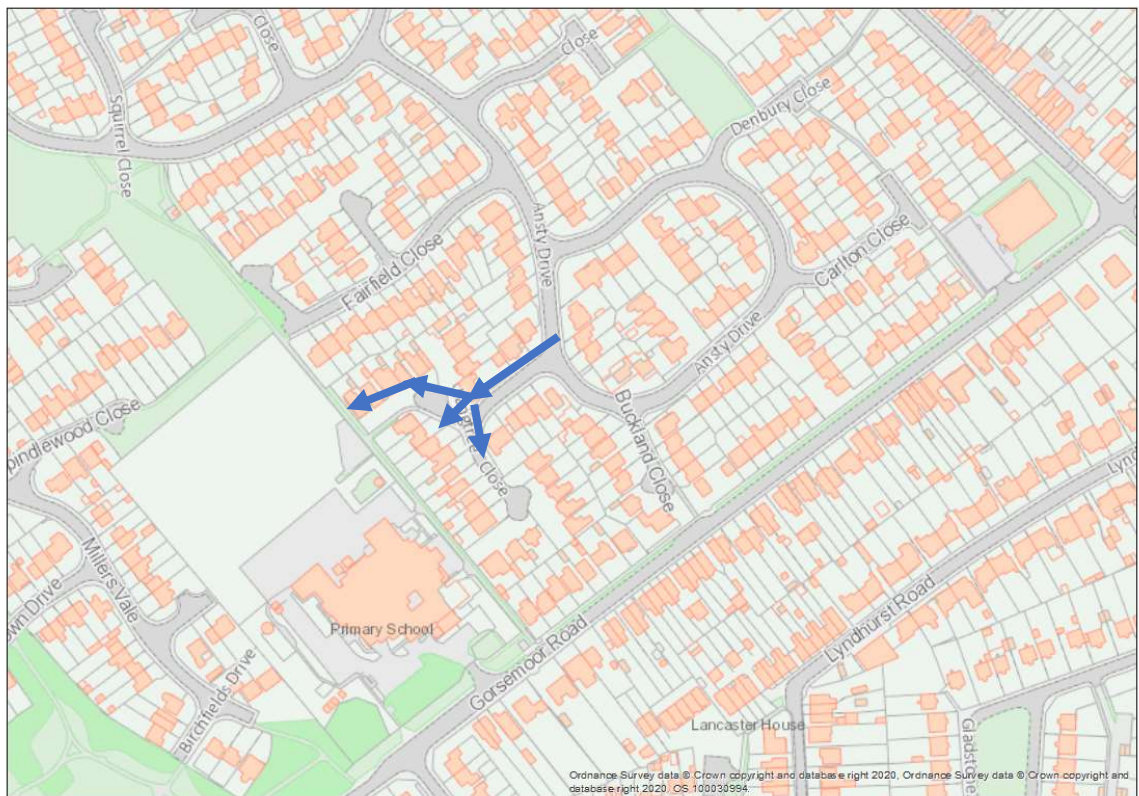
Figure 6- Surface water flow routes (blue arrows)
